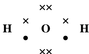
Water ( H_2O )
